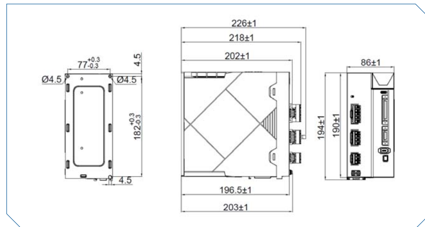
JSDG3-10B/15B/25B/35B(-E) (400V级)
