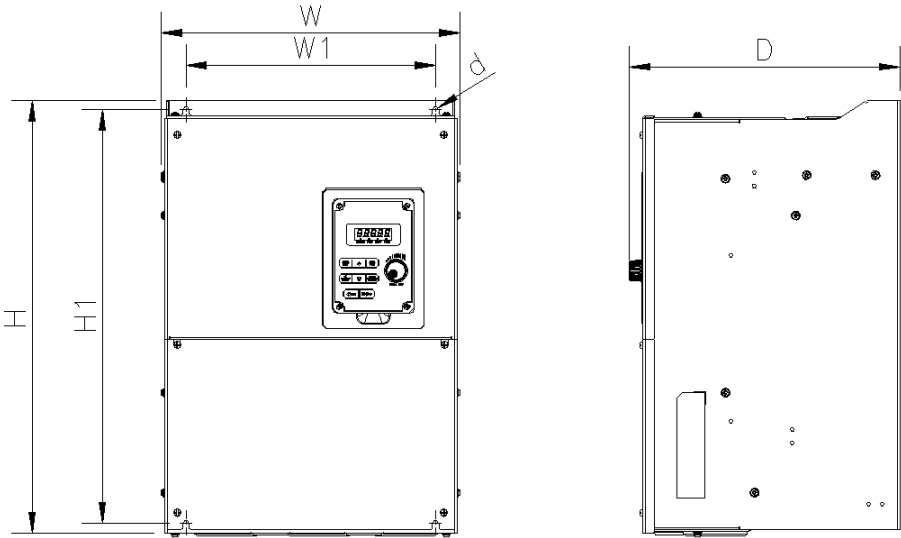
(c) 380V :25-30HP (IP20)
